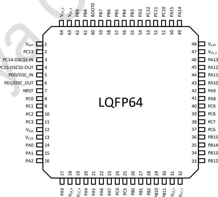
Figure 3-2 LQFP64 PY32F403R1xT Pinout1
