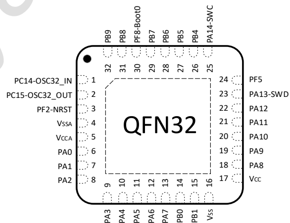
Figure3-5 QFN32(4*4) PY32F071K3xU7-E Pinout3 (Top view)
