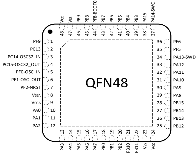
Figure 3-3 QFN48 PY32F040C1xU7-E Pinout1(Top view)
