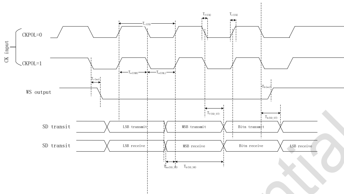
Figure 5-7 I²S timing diagram – Master mode(Philips protocol)
