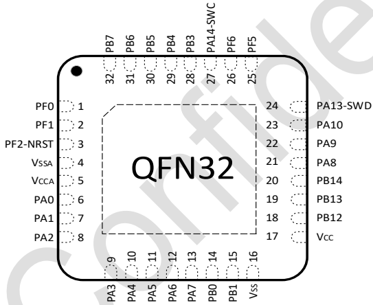
Figure 3-4 QFN32(4*4) PY32F040K2xU7-E Pinout2 (Top view)
