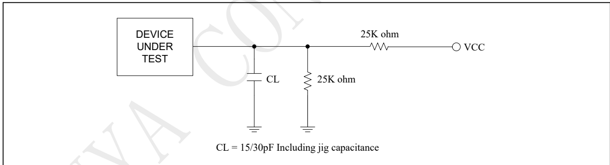
Figure 5-2 Output Loading
