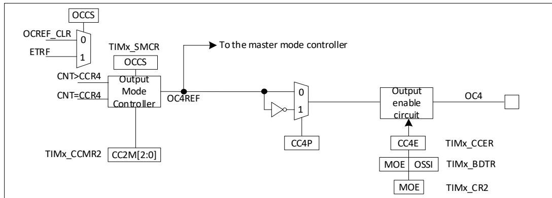
Figure 19-30 Output stage of capture/compare channel (channel 4)
