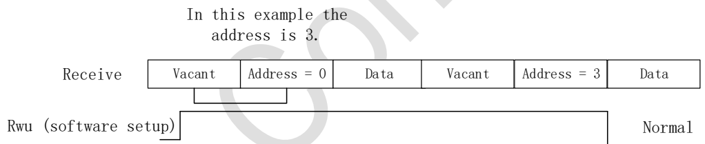
Figure 30-8 Slient mode with address tag detection
